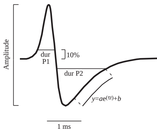
Fig. 2. Parameters measured in each digitized EOD waveform. Amplitude is measured peak-to-peak using cubic spline interpolation to improve accuracy. The duration of each phase (dur) is calculated 10% of the distance from the zero-crossing to the peak. The time constant \tau -P2 of the repolarization phase is estimated by fitting an inverse exponential to the middle 80% of the 2nd phase.
