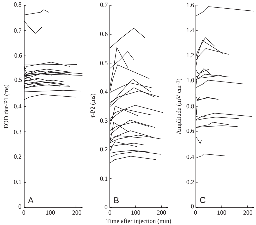
Fig. 8. Time courses of EOD duration and amplitude responses for 5-HT doses of 0.75 \text{ nmol g}^{-1} and higher. Points plotted are pre-injection baseline, 50% of peak, peak response, and response half-life. (A) Dur-P1 (duration of the first EOD phase) showed no clear response to 5-HT. (B) \tau -P2, (repolarization time of the second phase) showed the clearest response, with a bimodal distribution of peaks occurring at approx. 25 and 90 min after injection. (C) Amplitude was variable; if it rose, it peaked by approx. 30 min.
