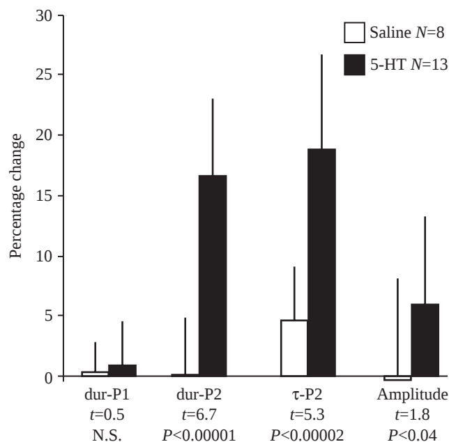
Fig. 6. Percentage change (mean \pm 1 s.d.) in responses of EOD waveform parameters to injection of serotonin at doses \geq 2.5 \text{ nmol g}^{-1} , or to saline controls. EOD parameters were measured as in Fig. 2. Means were compared with two-sample t -tests; the P values shown are one-tailed. Compared to the controls, serotonin caused significant increases in amplitude, second phase duration (dur-P2), and second phase repolarization time ( \tau -P2), but not of first phase duration (dur-P1).
