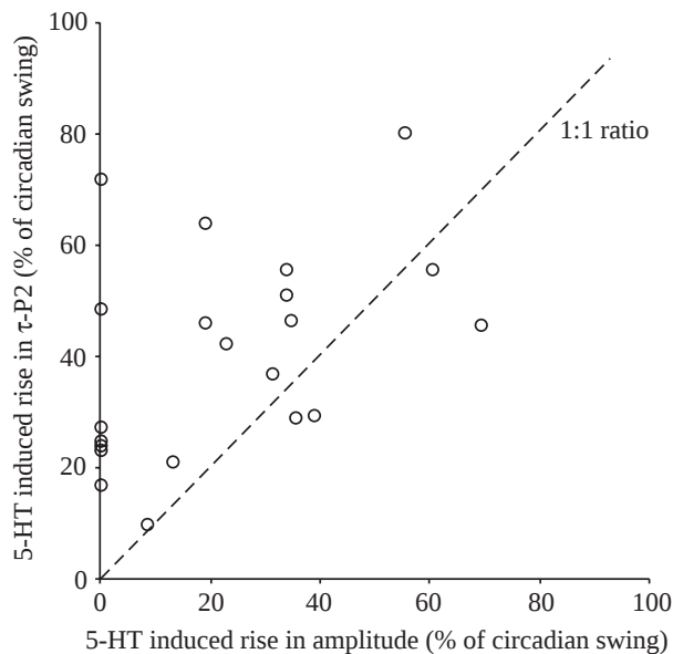
Fig. 9. 5-HT induced rise in EOD repolarization time ( \tau -P2) versus rise in amplitude, expressed as a percentage of the day-night swing, illustrates how the serotonin-induced changes in repolarization time and amplitude are semi-independent. Note that most of the data fall above the 1:1 ratio (broken) line, indicating that both variables may change or repolarization time may change alone, but amplitude never changes without a change in repolarization time. Values shown are for males injected with 5-HT doses 0.75 \text{ nmol g}^{-1} and higher.
