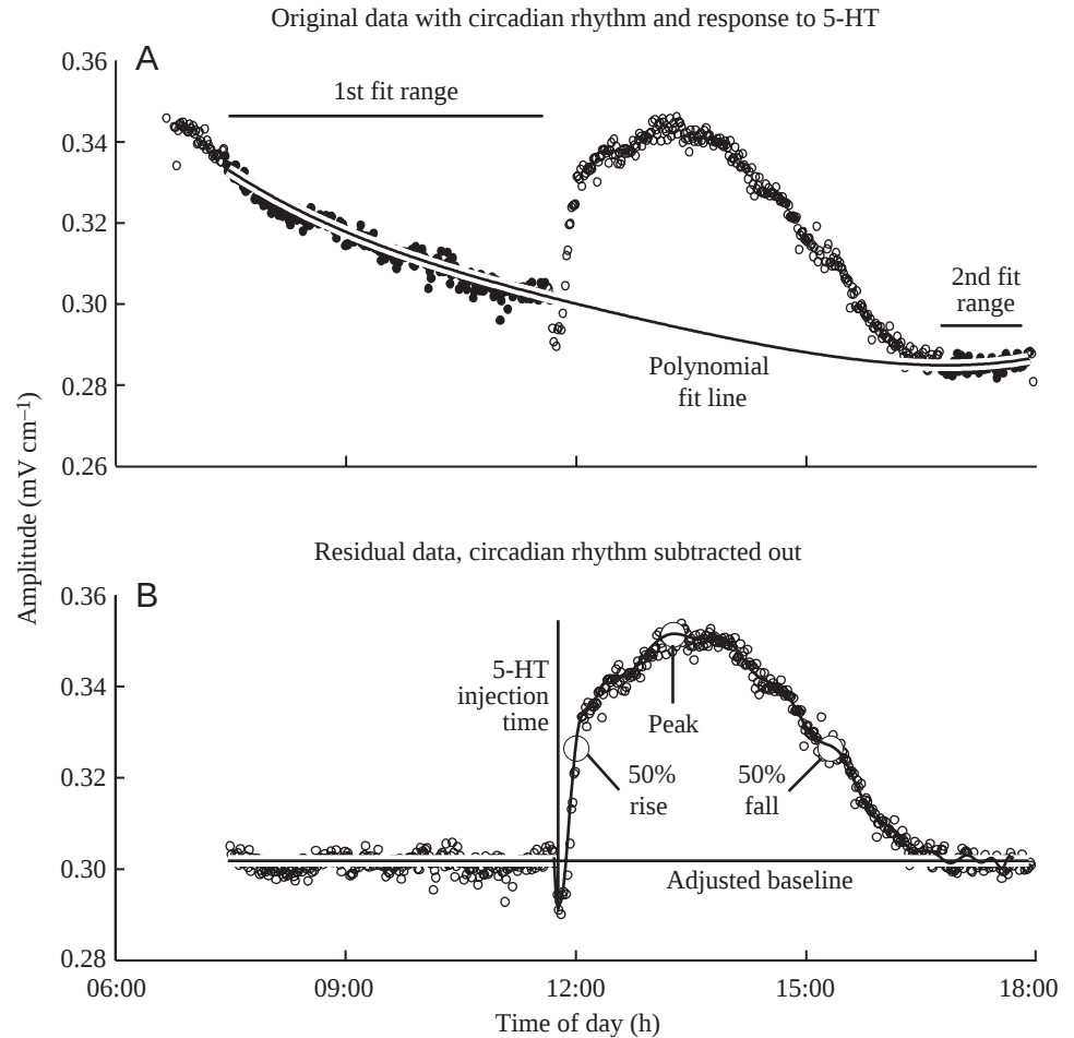
Fig. 3. Offline data analysis using polynomial regression to remove the circadian rhythm from the pharmacological response. (A) The raw data are shown with a fourth order polynomial least-squares regression fitted to segments of data before the injection and after the treatment had worn off. The polynomial is subtracted from the data to produce the residual data (B). A second, higher order polynomial is fitted to the residual data. The peak response and 50% peak response points are calculated for this polynomial.
